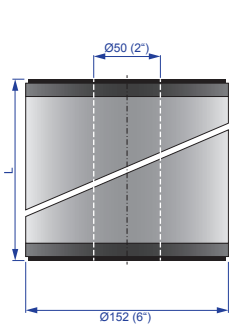
End Cap Design 1
