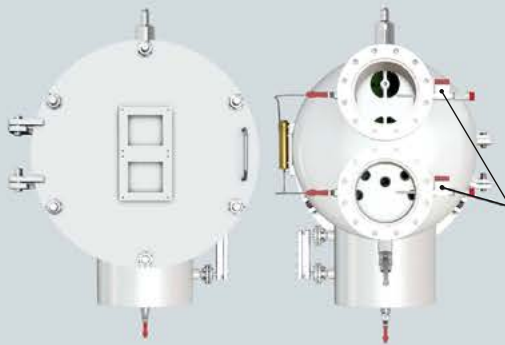
FAUDI Aviation 2 inch Coalescer and 4 inch Separator
